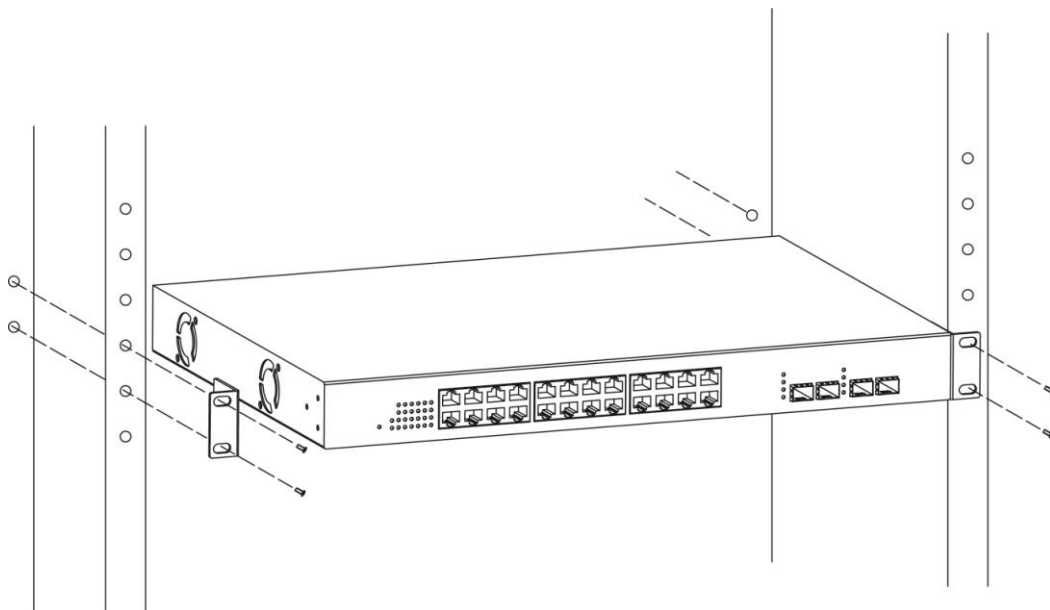
Rack-mount Installation
